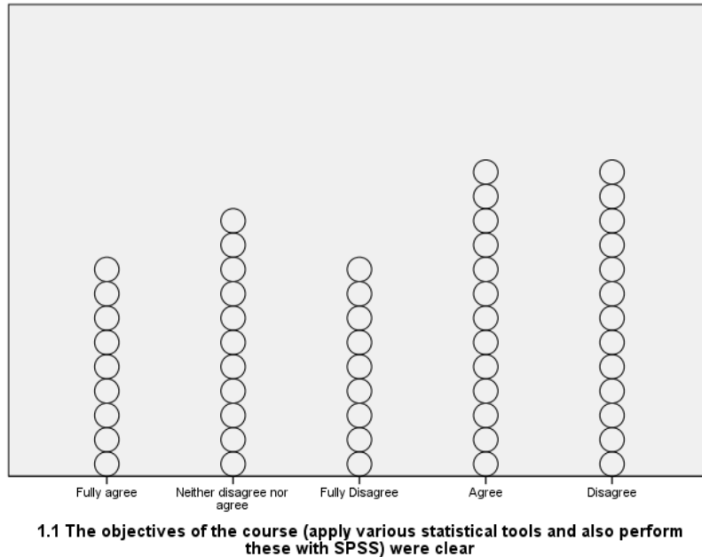
Figure 1. Example dot plot generated with SPSS
